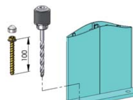
Floor Fixing
